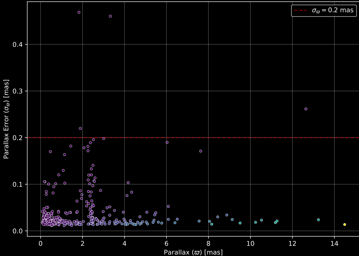
APOGEE DR17 Field: [ORIONB-A] Parallax Quality (n= 334)
