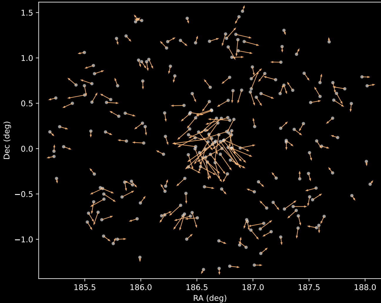
APOGEE DR17 Cluster 3 Proper Motion Vectors (n=226)
