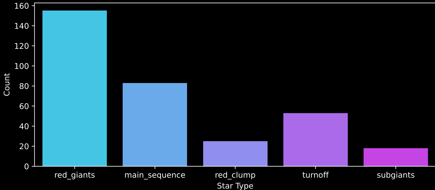
APOGEE DR17 Field: [ORIONB-A] Count plot of Star Type
