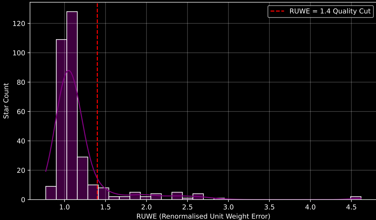
GAPOGEE DR17 Field [ORIONB-A] RUWE Distribution (n= 321)
