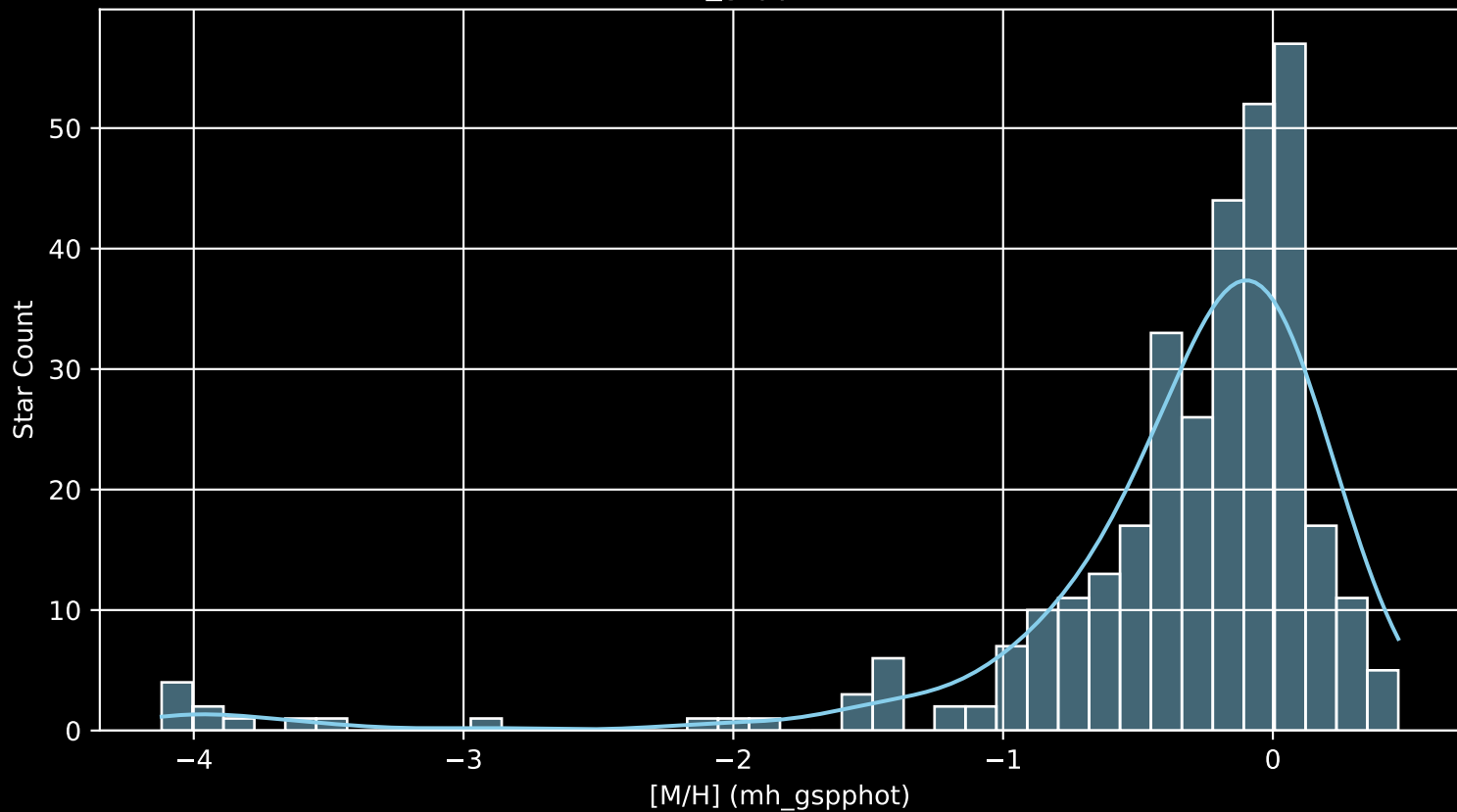
APOGEE DR17 Field: [ORIONB-A [M/H] (mh_gspphot) (n= 329)
