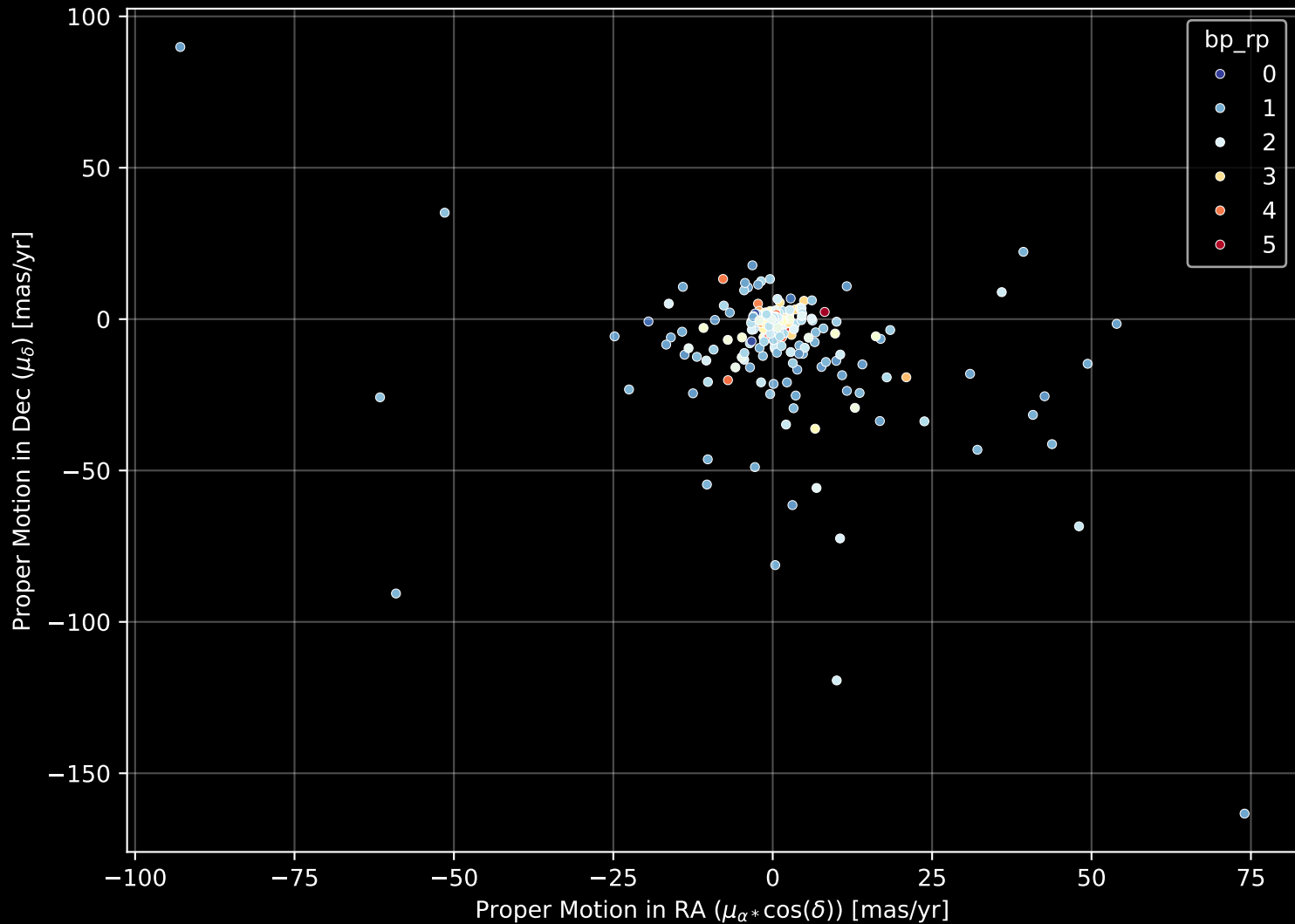
APOGEE DR17 Field: [ORIONB-A] Proper Motion Diagram (n= 334)
